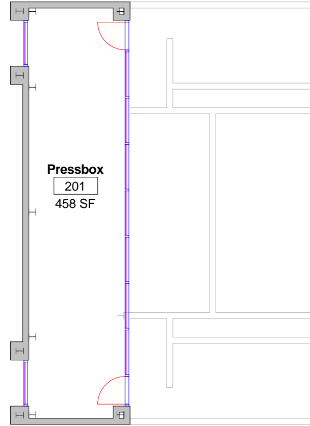
② Press Box Level 2 3/32" = 1'-0"
