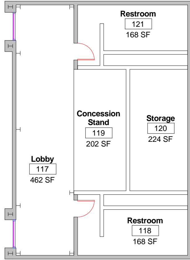
① Concessions/Restrooms Level 1 3/32" = 1'-0"
